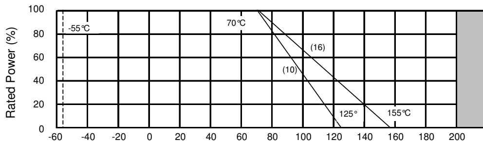
Fig.1 Power Derating Characteristics
