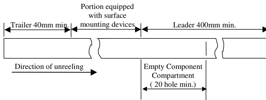
Fig. 2 Explanation of Leader and Trailer Tape
